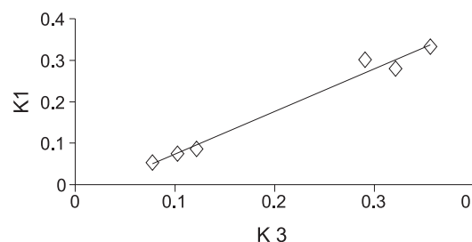
Figure 5. A linear plot for the relationship between the first-order dissolution rate constant ( K_1 ) and the Hixson-Crowell cube root dissolution rate constant ( K_3 ).
